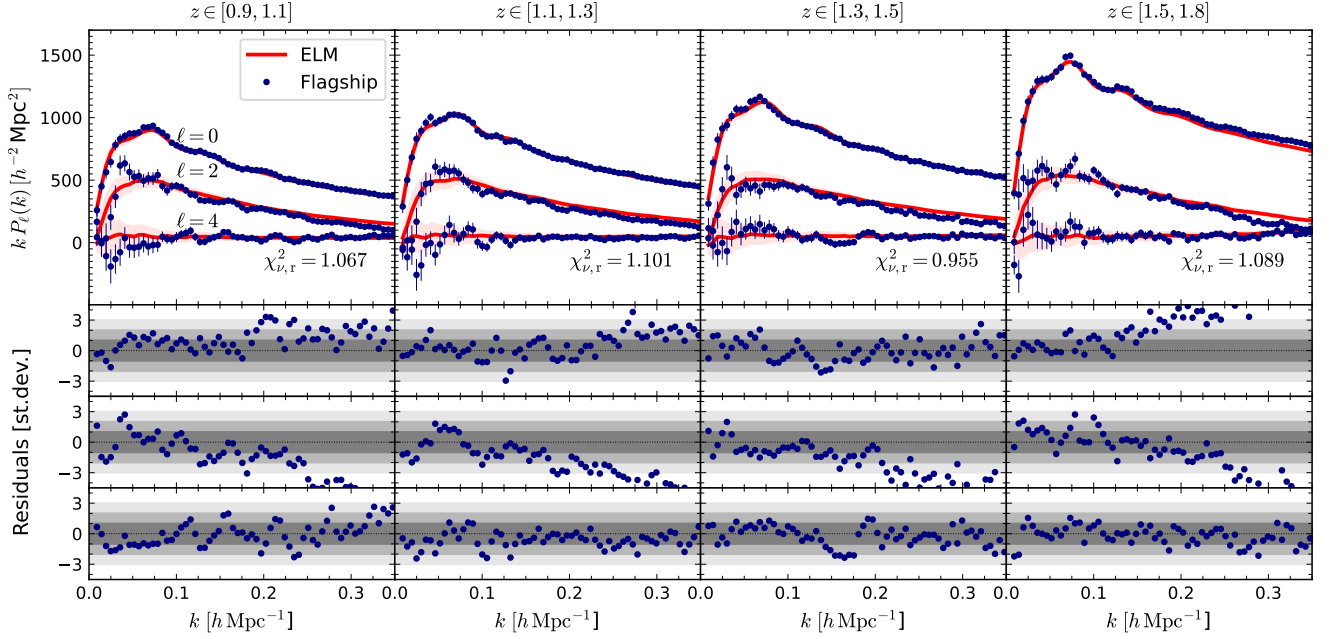
Fig. 8. Power spectrum multipoles of galaxies with f_{\text{H}\alpha} > f_0 for Flagship (blue points) and EuclidLargeMocks (red lines) in the four redshift bins, as indicated at the top of each column of panels. The lower panels show the residuals of the Flagship measurements (from top: monopole, quadrupole, hexadecapole) with respect to the average EuclidLargeMocks in units of the standard deviation of the latter.
