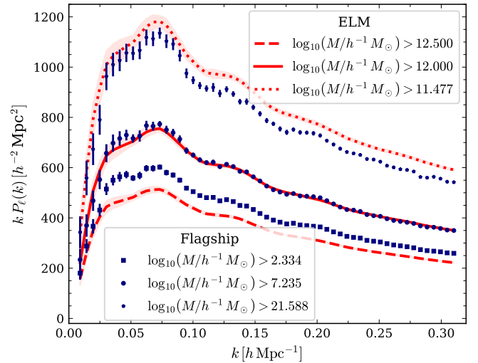
Fig. A.2. Power spectrum monopole of halos, with z \in [0.9, 1.1] , in the Flagship mock and in 50 EuclidLargeMocks for three distinct mass cuts that obey the CM relation.
