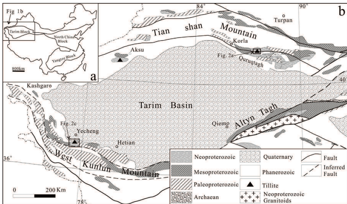
Fig. 1. (a) Schematic tectonic map of China showing the three major Precambrian blocks. (b) Sketch map of the Tarim block and adjacent areas showing the Precambrian geology and surrounding orogens (after Lu et al., 2008).
