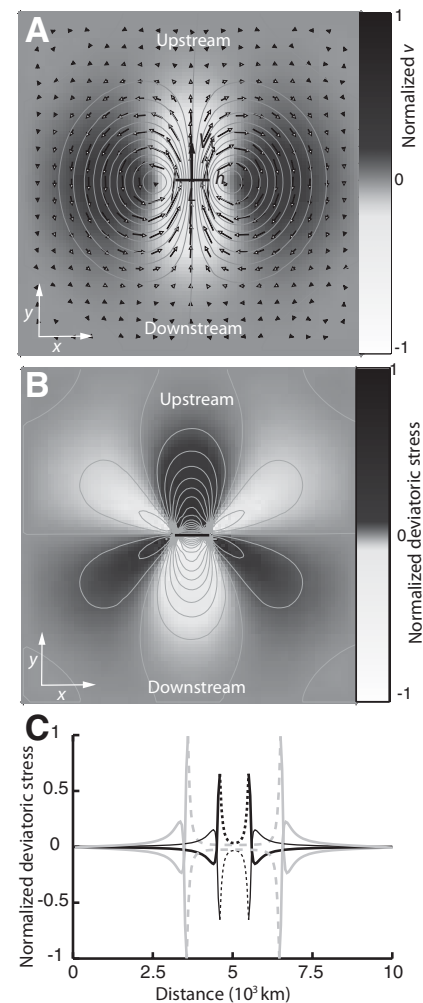
Figure 1. Map view of model. A: Normalized streamlines (gray curves), velocity field (arrows), and v , velocity field, parallel to y axis (background). V_r is translation velocity of slab. L and h are slab width and thickness. B: Normalized deviatoric stress, iso-curves every 0.05. C: Deviatoric stress profile along line parallel to x axis and running on upstream (bold) and downstream (thin) side of 1000 km (black) and 3000 km (gray) plate across model. Dashed sections denote stresses along slab.
