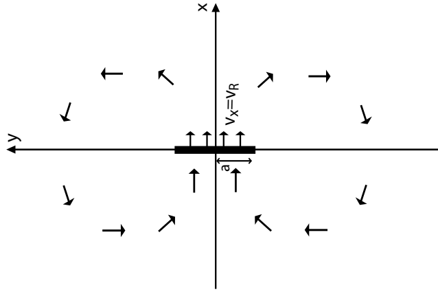
Figure 3. Plan view of Hele-Shaw flow field used to approximate viscous pressure of toroidal flow around a slab of half-width a , moving in the horizontal plane at a rate v_R .
