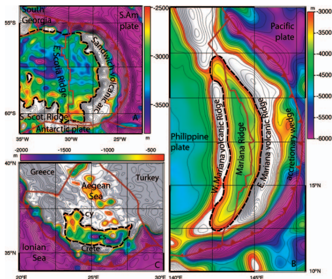
Figure 1. Topography of East Scotia (A), Mariana (B), and Aegean (C) seas (wavelengths <50 km are discarded). Deflection of topography toward center of basins can be pointed out by circumscribing (dashed lines) areas deeper than arbitrary reference depth in overriding plates (A, 2500 m; B, 3000 m; C, 350 m). Isocontours are every 250 m. S. Am.—South American Plate; S.Scot—South Scotia.
