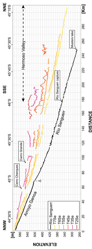
Figure 9. Topographic longitudinal profiles of the fluvial terraces of the Rio Senguerr system.
