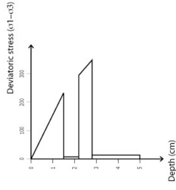
Figure 2.: Strength profiles for the experimental lithosphere and the heterogeneity.
