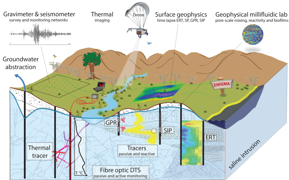
Figure 19: Co-location of different imaging techniques on densely monitored experimental sites to quantify subsurface spatial structures, fluxes, heat transfer and reactive transport phenomena (ENIGMA network proposal, see perspective section).
