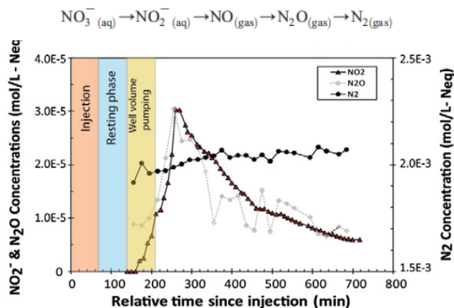
Figure 17: Results of the reactive pushpull test experiment: breakthrough curves for the reaction by-products NO_2^- , N_2O , and N_2 (H+ Ploemeur test site).
