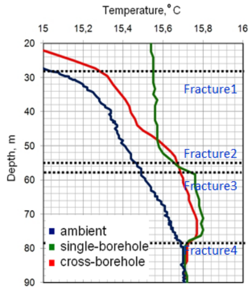
Figure 21: (A) Temperature profiles in B2 (H+ Ploemeur test site) measured under different flow conditions. The blue curve presents temperature profile under ambient flow. The green curve was collected while pumping with pumping at the top of B2 with a pumping rate Q = 125 l/min. The red curve corresponds to the cross-hole pumping test while pumping was turned on in B3 with a pumping rate Q = 145 l/min.
