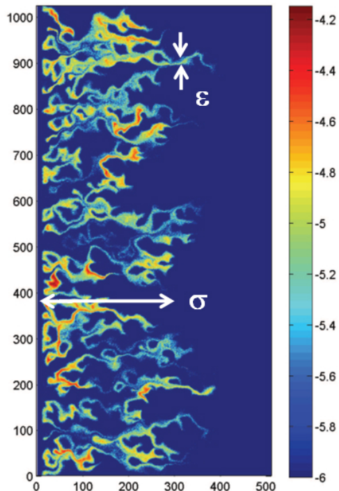
Figure 5: Concentration field simulated in a heterogeneous Darcy field (as in figure 1), illustrating the difference between the spreading scale \sigma that describes the spatial extent of the plume and the mixing scale \epsilon that quantifies the scale at which solutes can be assumed to be fully mixed (adapted from Le Borgne et al. (2010)).
