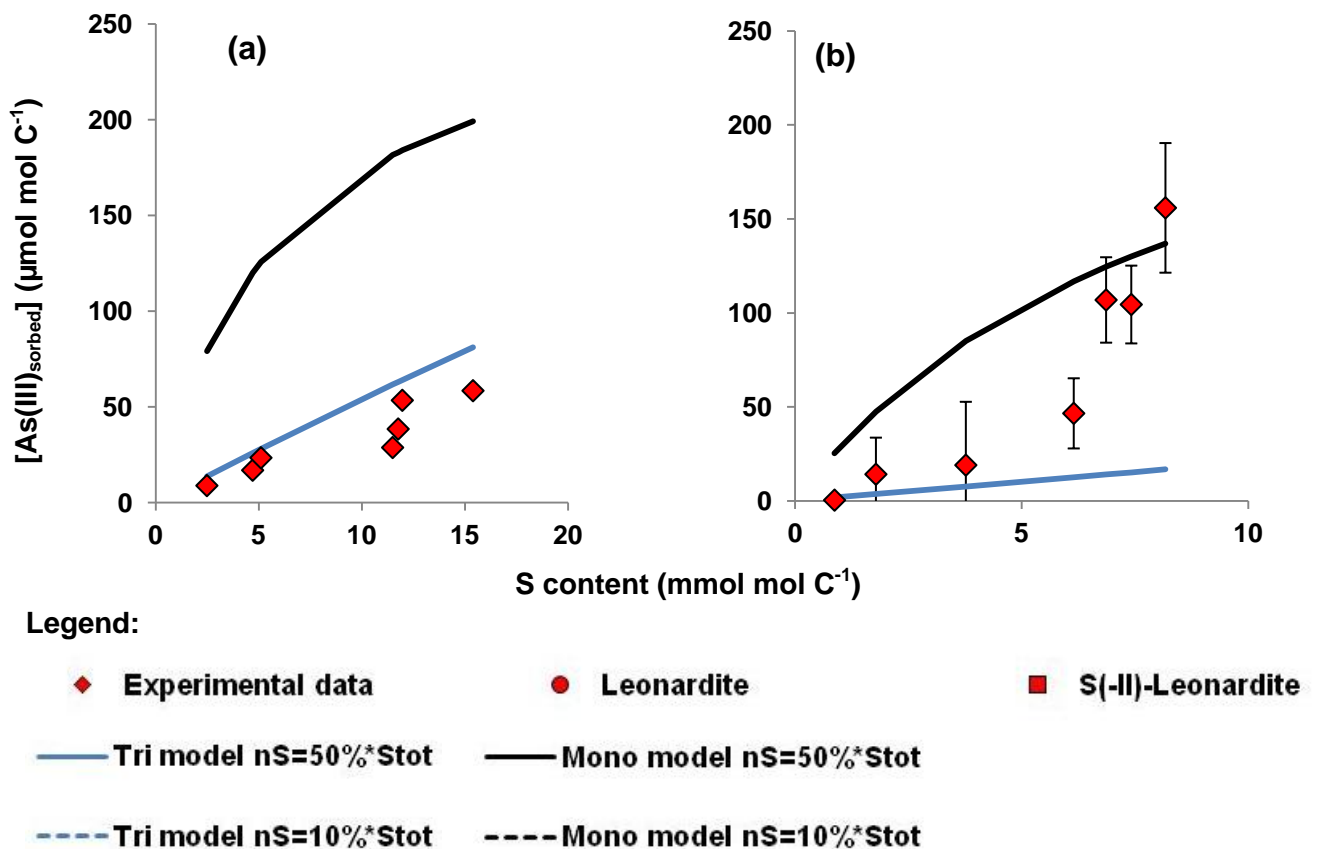
Figure I. 7: Experimental and modeled datasets of (a) HA experimental data from Hoffmann et al. (2012), (b) peat experimental data from Hoffmann et al. (2012).
