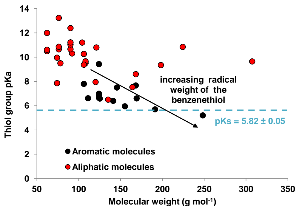
Figure I. 8: Compilation of the pKa of the thiol function of thiol-containing organic molecules according to their molecular weight (Edsall and Wyman, 1958; Gough et al., 2003; Martell and Smith, 1989; Williams, n.d.). The distinction was made between aliphatic (red symbols) and aromatic ring-containing molecules (black symbols).
