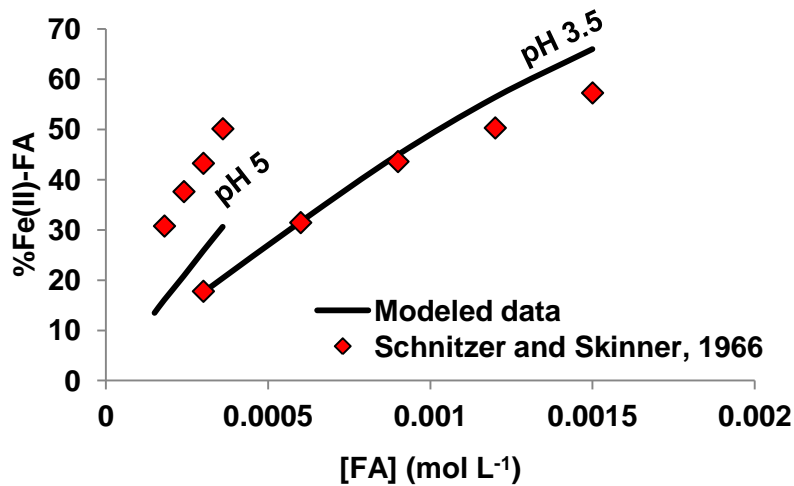
Figure II. 6: Schnitzer and Skinner's (1966) dataset: experimental and modeled % of Fe(II) adsorbed onto FA.
