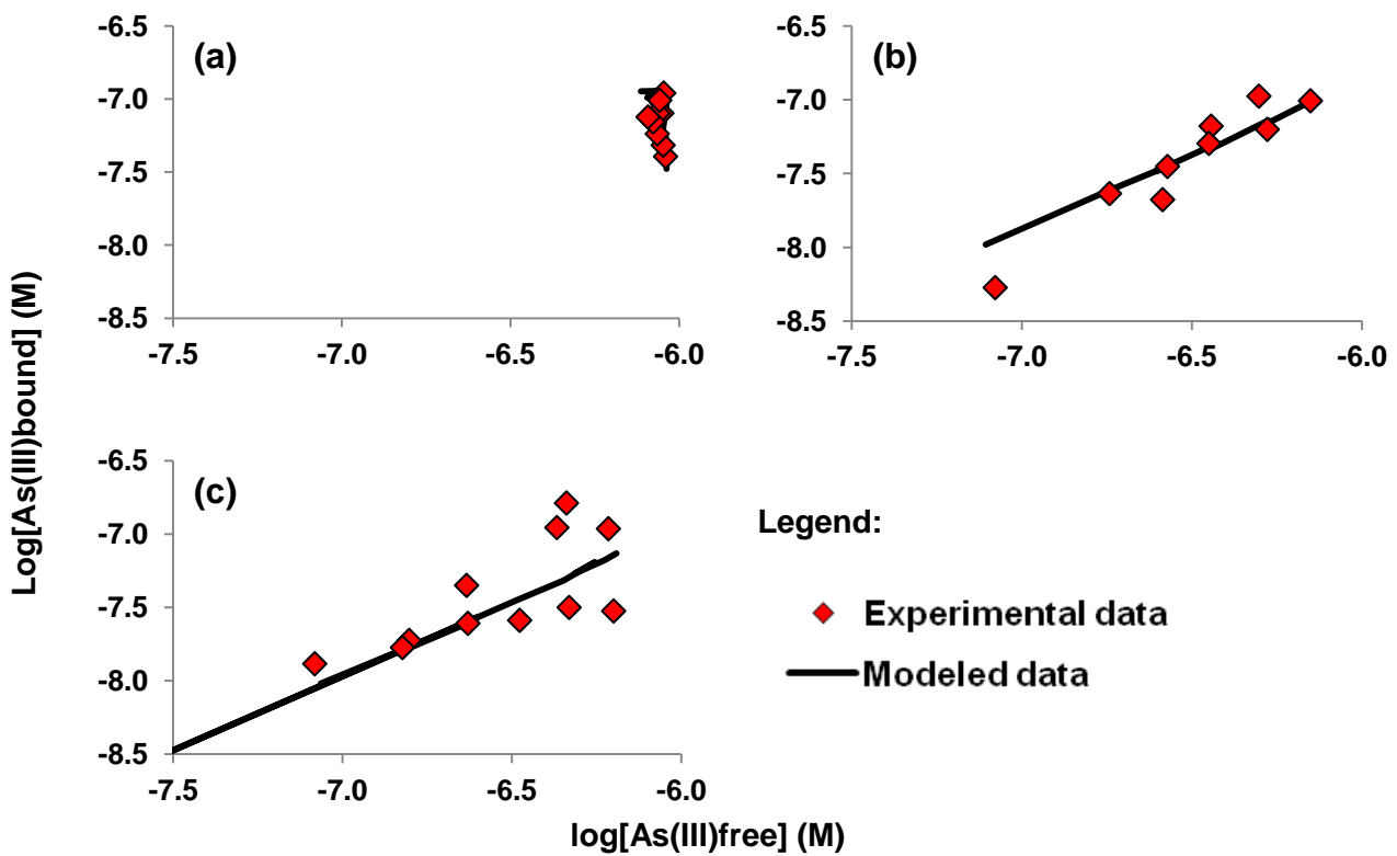
ANNEXE III 10: Sum of Eq.3 + Eq. 4 (a) isotherm with increasing Fe(II) concentrations at pH 6, (b) isotherm with increasing As(III) concentrations at pH 6, (c) isotherm with increasing Fe(II) concentrations at pH 5.
