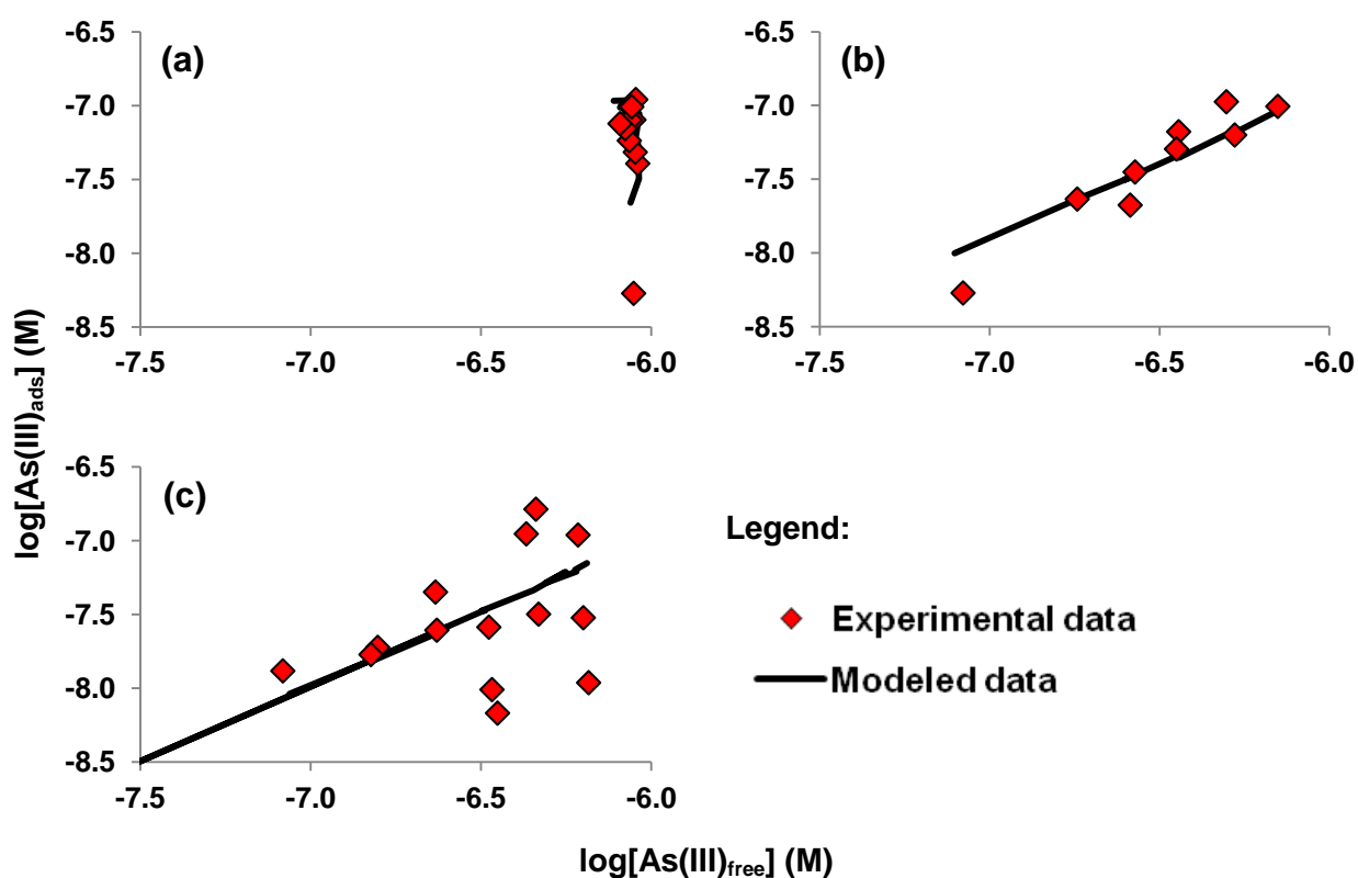
Figure III. 3: Sum of Eq.3 + Eq. 4 + Eq.5 + Eq. 6 (a) isotherm with increasing Fe(II) concentrations at pH 6, (b) isotherm with increasing As(III) concentrations at pH 6, (c) isotherm with increasing Fe(II) concentrations at pH 5.
