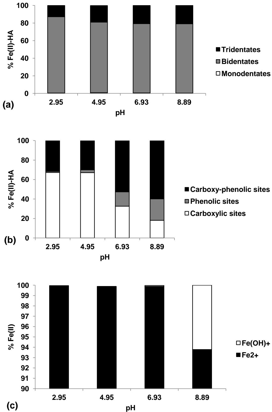
Figure II. 5: Fe(II) speciation onto the binding sites - pH adsorption edge - DOC = 76 mg L -1 (a) Denticity, (b) Type of site, (c) Form of adsorbed Fe(II).
