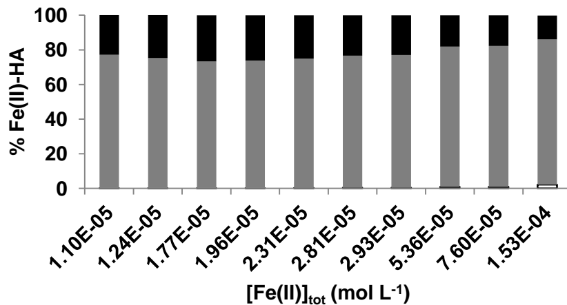
(a) Monodentates Bidentates Tridentates
