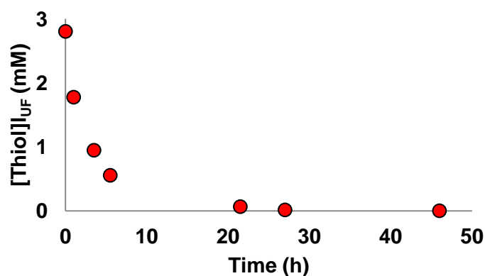
Figure I. 1: Thiol group grafting ( \text{mmol L}^{-1} ) over time expressed in hours
