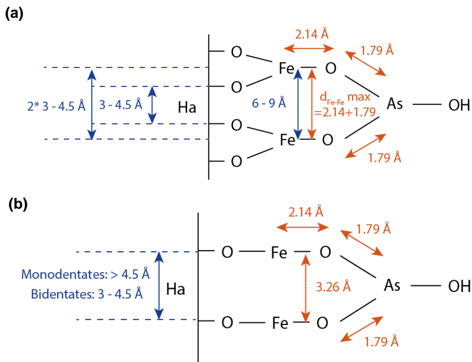
Figure III. 5: Complexes formed with (a) Eq. 6 and (b) Eq. 4. Fe-O and As-O distances (in red) were determined from the \text{Fe}(\text{OH})_2 oxides and \text{As}(\text{OH})_3 , respectively (Ona-Nguema et al., 2009). The distances in blue are defined in PHREEQC-Model VI (Tipping, 1998).
