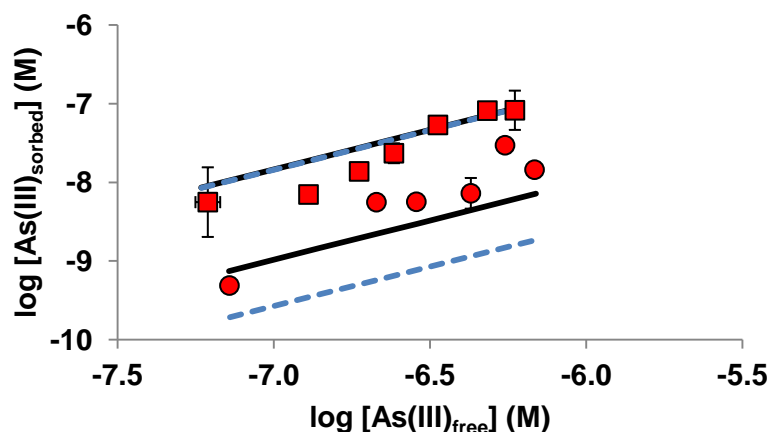
Figure I. 3: Experimental and modeled datasets of Leonardite and S(-II)-Leonardite
