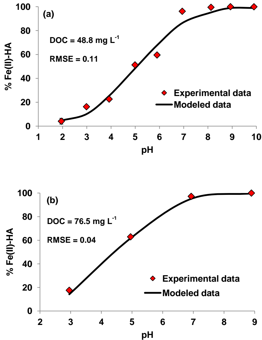
Figure II. 2: (a) pH adsorption edge - DOC = 50 mg L -1 (b) pH adsorption edge - DOC = 76 mg L -1 (the error bars calculated from the triplicated experiments are within the symbols.). As each experiment was performed in triplicate, each point represents the average of the triplicates. The error bars represent the standard deviation (in log or percentage, depending on the data) calculated from the triplicated experimental data.
