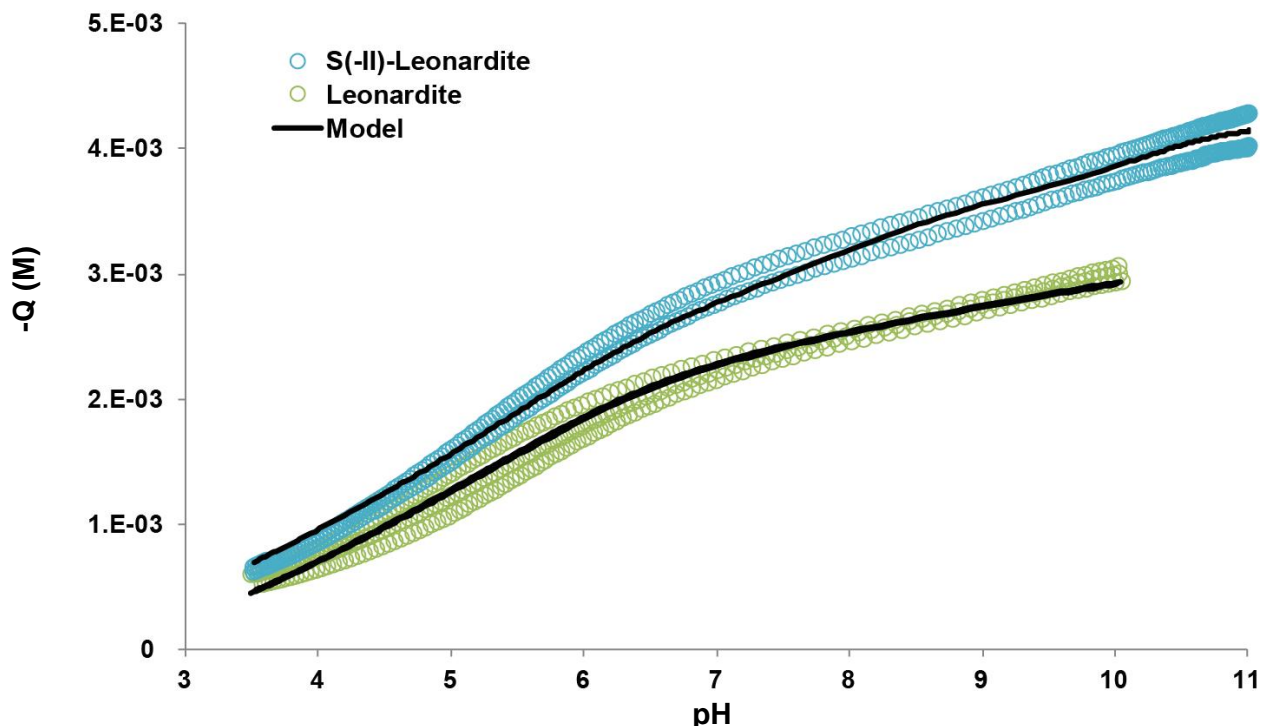
Figure I. 2: Titrations of Leonardite (shown as green symbols) and S(-II)-Leonardite (shown as blue symbols) as compared to the modeling (shown as black lines).
