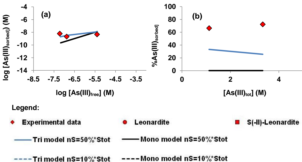
Figure I. 6: Experimental and modeled data (Mono = with monodentates only; Tri = with tridentates only) (a) SRHA experimental data from Kappeler (2006), (b) SRHA experimental data from Figure 1 of Lenoble et al. (2015)
