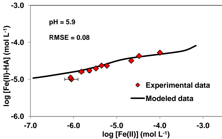
Figure II. 1: Adsorption isotherm: experimental and modeled data
