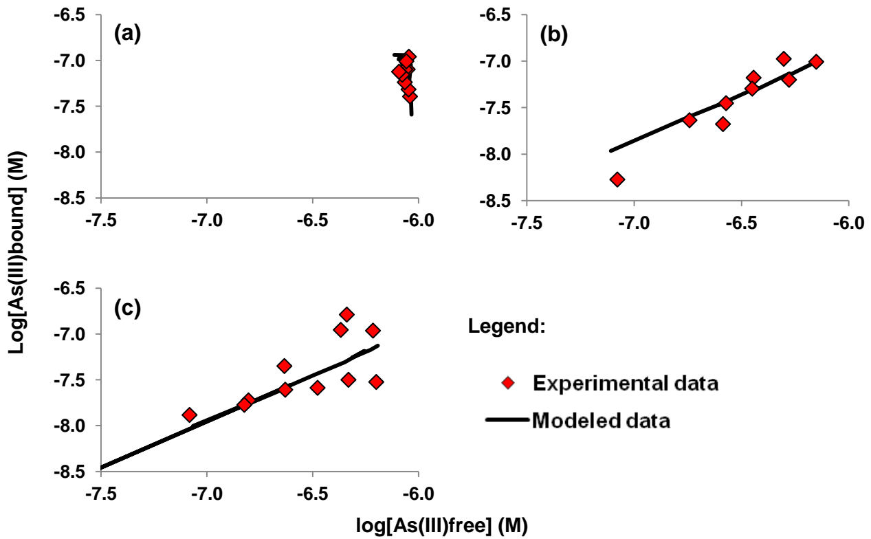
ANNEXE III 8: Formation of As(III) binuclear monodentate to Fe(II) bidentate with OM (a) isotherm with increasing Fe(II) concentrations at pH 6, (b) isotherm with increasing As(III) concentrations at pH 6, (c) isotherm with increasing Fe(II) concentrations at pH 5.
