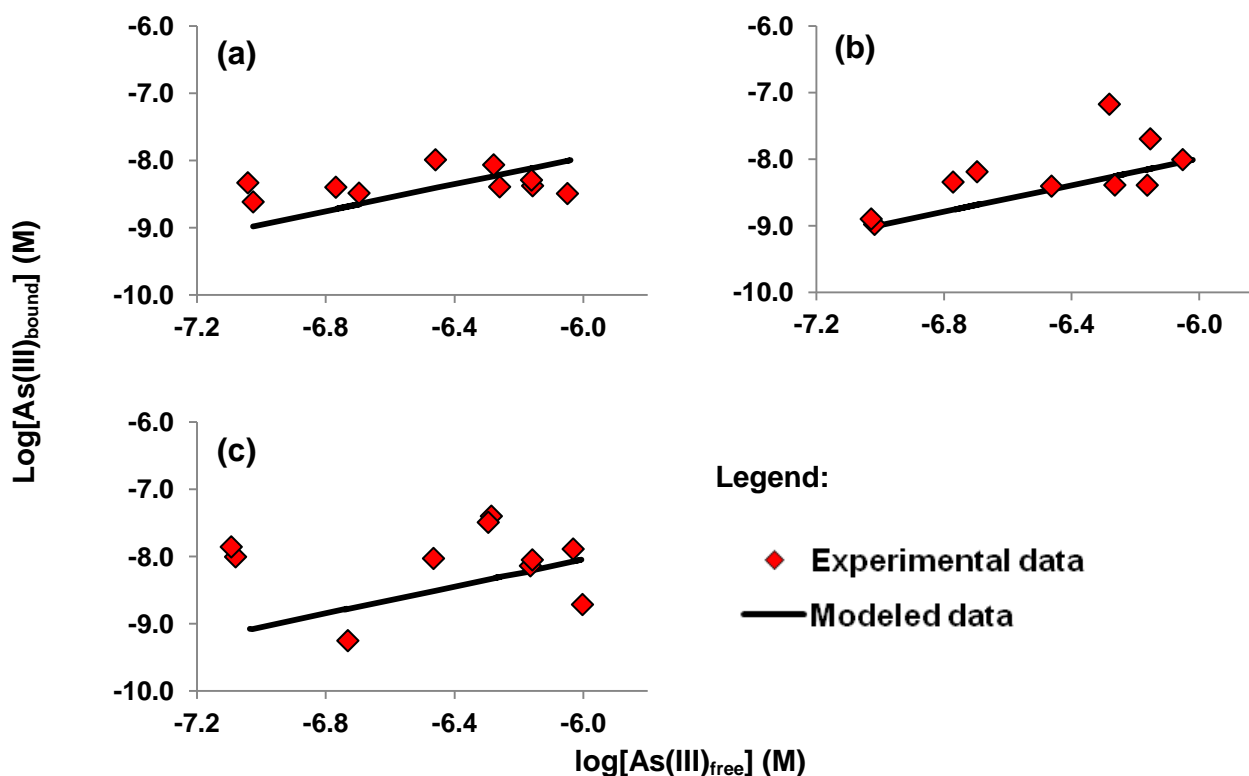
Figure III. 4: As(III)-Fe(III)-HA binding experiments and modeled data using only thiol binding parameters at (a) pH 4, (b) pH 5, (c) pH 6.
