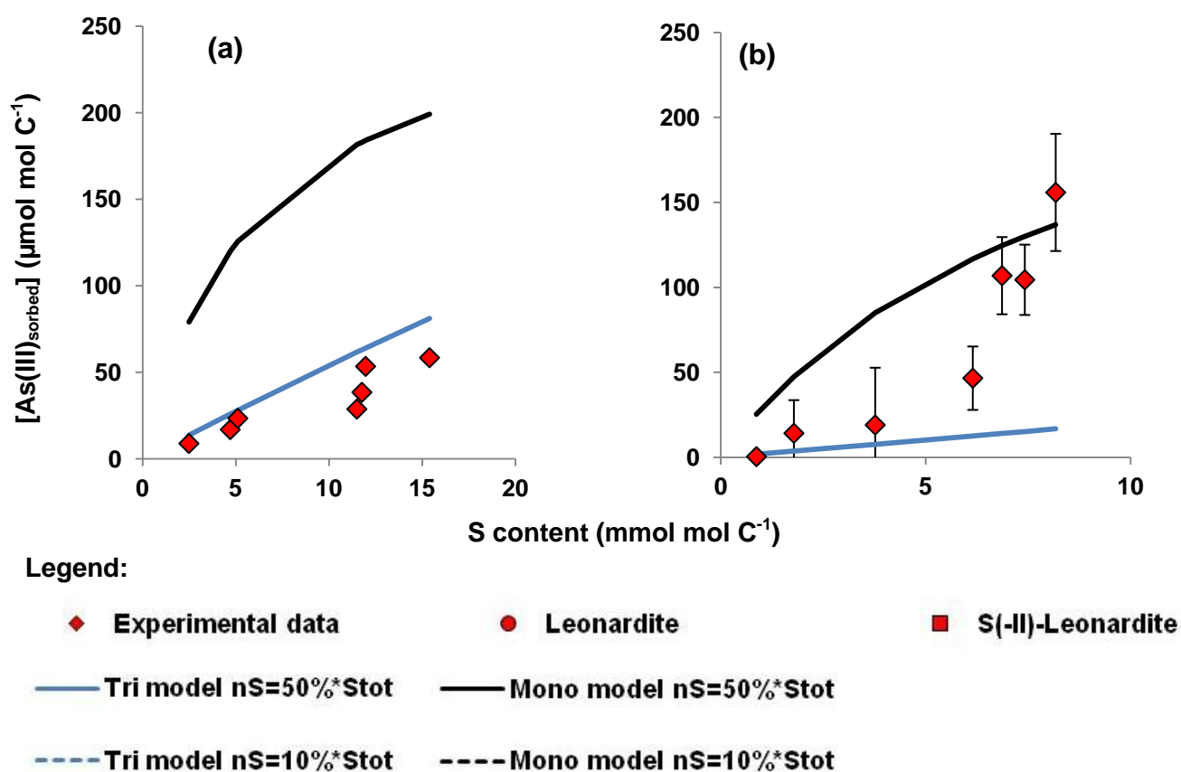
Figure I. 7: Experimental and modeled datasets of (a) HA experimental data from Hoffmann et al. (2012), (b) peat experimental data from Hoffmann et al. (2012).
