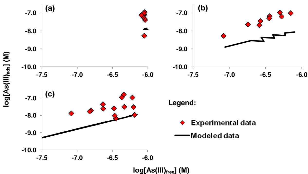
Figure III. 2: As(III)-Fe(II)-HA binding experiments and modeled data using only thiol binding parameters (a) according to the [\text{Fe(II)}] concentration, (b) at pH 6, (c) pH 5.
