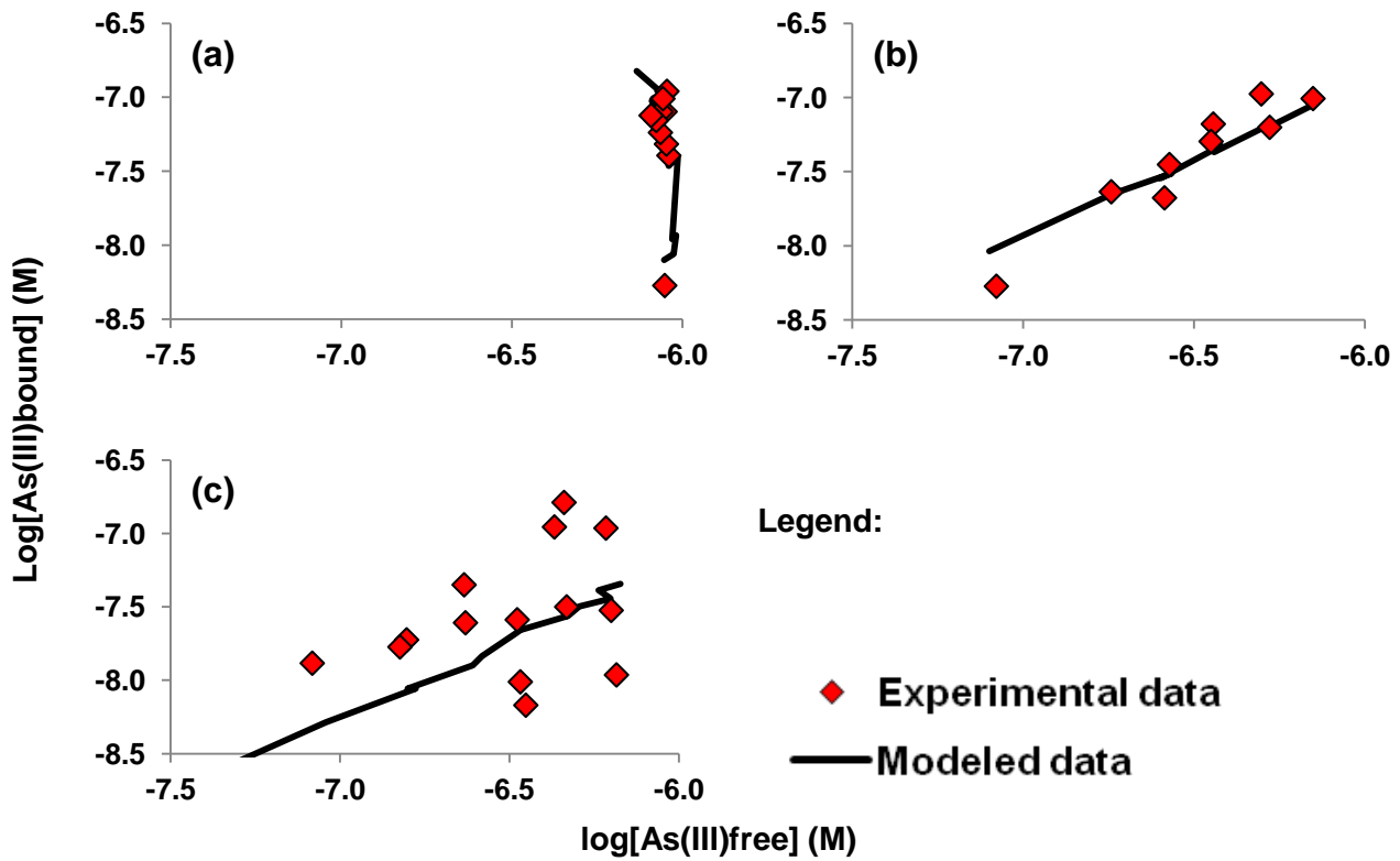
ANNEXE III 9: Sum of Eq.1 + Eq. 2 (a) isotherm with increasing Fe(II) concentrations at pH 6, (b) isotherm with increasing As(III) concentrations at pH 6, (c) isotherm with increasing Fe(II) concentrations at pH 5.
