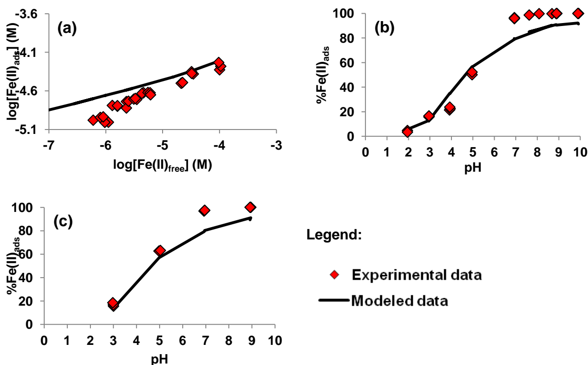
Figure III. 1: (a) Experimental and modeled adsorption isotherm of Fe(II) to HA (b) pH adsorption edge — DOC = 50 mg L -1 , (c) pH adsorption edge — DOC = 76 mg L -1 .
