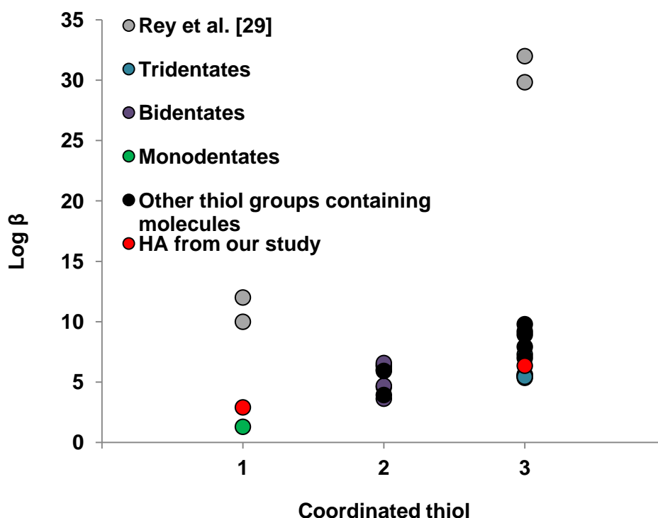
Figure I. 9: Comparison between \log \beta of thiol-containing organic molecules and As(III) and \log K_{MS} relative to the number of coordinated thiols in the complexes (Cavanillas et al., 2012; Gaber and Fluharty, 1972; Hoffmann et al., 2014; Rey et al., 2004; Spuches et al., 2005b; Spuches and Wilcox, 2008; Starý and Růžicka, 1968; Zahler and Cleland, 1968; Zhao et al., 2012).
