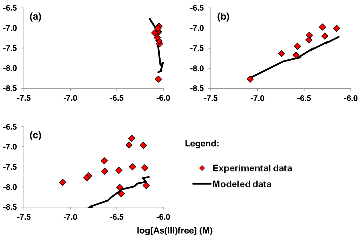
ANNEXE III 4: Formation of As(III) binuclear monodentate to Fe(II) monodentate with OM (a) isotherm with increasing Fe(II) concentrations at pH 6, (b) isotherm with increasing As(III) concentrations at pH 6, (c) isotherm with increasing Fe(II) concentrations at pH 5.
