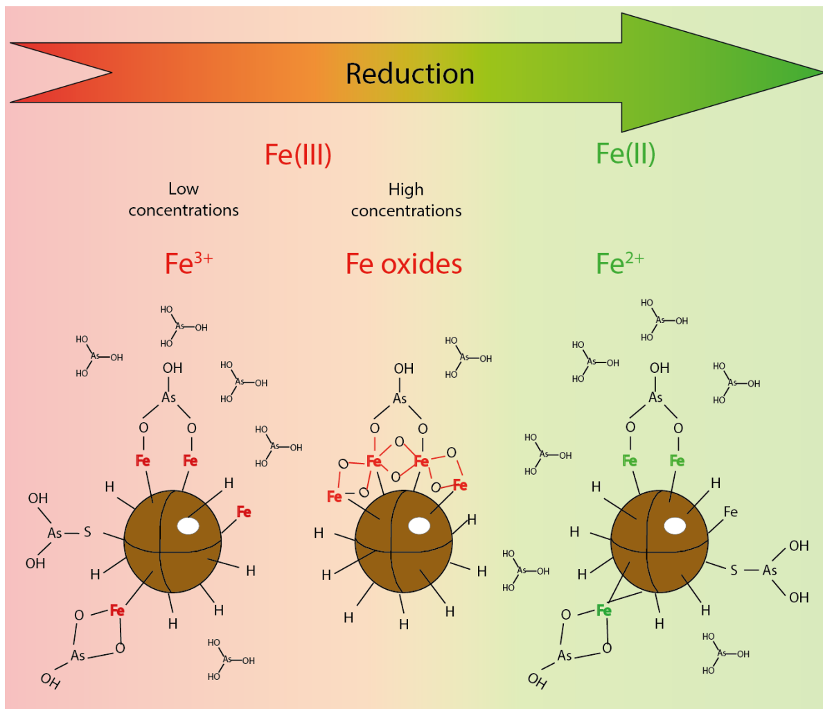
Figure III. 7: Schematic model describing the different complex types that may form between \text{As}(\text{III}) , \text{Fe}(\text{II}) and/or \text{Fe}(\text{III}) and dissolved organic matter (DOM), depending on the redox status of Fe, and on Fe and DOM concentrations. This general scheme may apply to what happens in floodplain and wetland waters (Catrouillet et al., 2015; Hoffmann et al., 2013; Mikutta and Kretzschmar, 2011).
