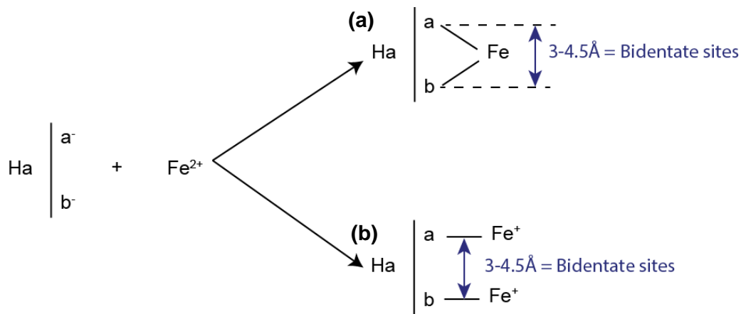
Figure III. 6: Bidentate sites defined in (a) a bidentate mode (actual definition in PHREEQC-Model VI) and (b) a monodentate mode (new definition).
