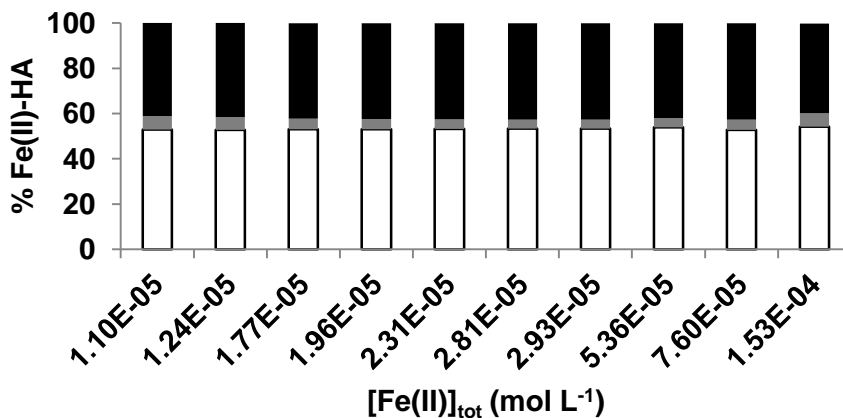
(b) Carboxylic sites Phenolic sites Carboxy-phenolic sites
