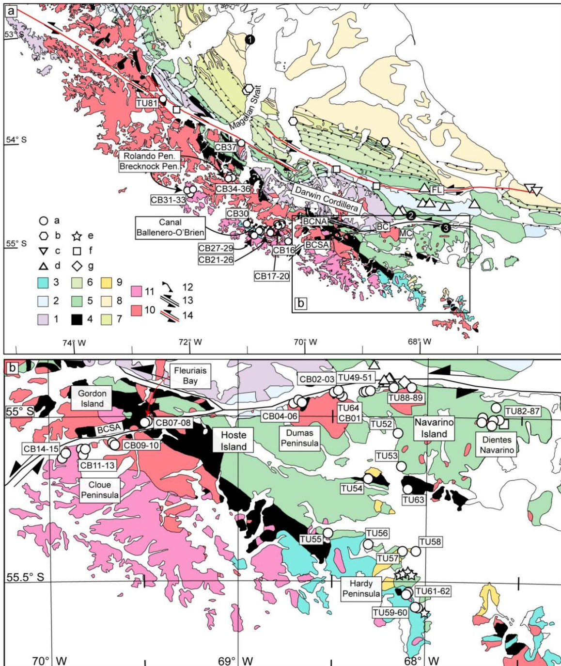
Figure 3: a) Simplified geological map of the southern tip of South America (modified from Alvarez-Marrón et al. (1993); Hervé et al. (1984); Klepeis (1994b); Mpodozis and Rojas (2006); Olivero and Malumián (2008); SERNAGEOMIN (2003); Suárez et al. (1985)). Main cities are shown in black circles: 1, Punta Arenas; 2, Ushuaia and 3, Puerto Williams; FL, Fagnano Lake; BC, Beagle Channel; MC, Murray Channel. Legend of the geological maps: 1, Paleozoic Basement; 2, Jurassic magmatism; 3, Cretaceous volcanism; 4, Ophiolitic complexes; 5, Lower Cretaceous sedimentary sequences; 6, mid-Upper Cretaceous sedimentary sequences; 7, Upper Cretaceous-Paleocene sedimentary sequences; 8, Eocene-Pliocene sedimentary sequences; 9, Miocene volcanics; 10, Cretaceous intrusive rocks; 11, Paleocene intrusive rocks; 12, thrust faults; 13, Beagle Channel fault zone; 14, Magallanes-Fagnano fault zone. Paleomagnetic sampling of this study and previous published paleomagnetic results are shown in white symbols (a, this study; b, Poblete et al., 2014; c, Maffione et al., 2010; d, Rapalini, et al., 2015; e, Cunningham et al., 1991; f, Burns et al., 1980; g, Dalziel et al., 1973). b) Inset showing the area of the Beagle Channel, Isla Navarino and Hardy Peninsula. Color legend is as in Fig. 3a.
