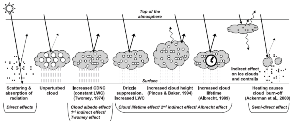
Figure 1-5 – Main radiative effects of atmospheric aerosols, based on Haywood and Boucher (2000).
