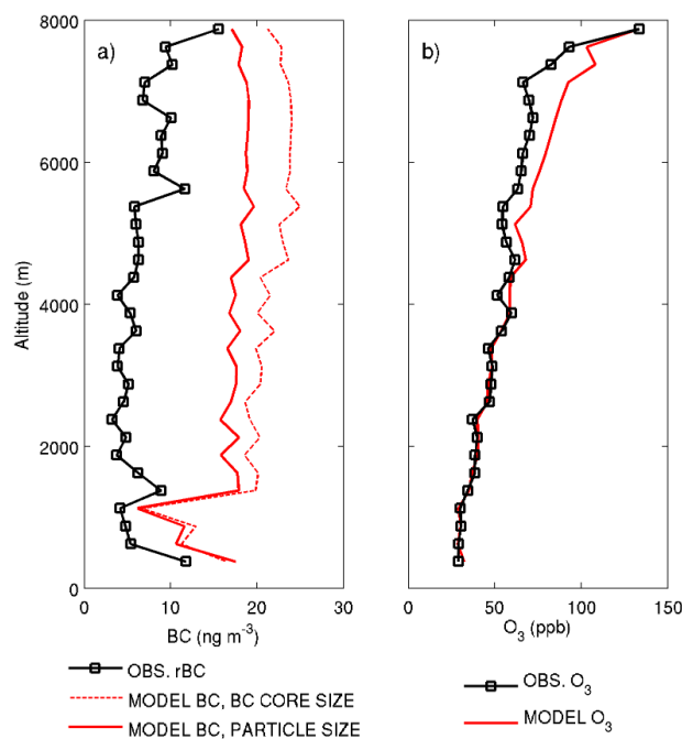
Figure 6-4 – Mean (a) SP2 rBC and (b) \text{O}_3 profiles from the ACCESS aircraft campaign (black, July 2012, Northern Norway) compared to WRF-Chem BC and \text{O}_3 interpolated along ACCESS flights (base simulation). SP2 rBC measurements cover the size range 80 to 470 nm, and WRF-Chem 80 to 470 nm BC was calculated in two ways 1) from the size distribution of the internally mixed particles in MOSAIC (thick continuous red line) and 2) by estimating the size of BC “cores” within each MOSAIC size bin (thin dotted red line)
