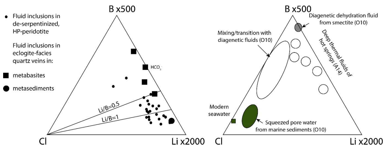
Figure 42 : B and Li concentration in fluids from variable depth domains, down to eclogite-facies conditions, adapted from (Yoshida et al., 2015). In the left diagram, corresponding to high pressure domain, fluids were analyzed in fluid inclusions in olivine by LA-ICP-MS (small circles) (Scambelluri and Philippot, 2004), and in eclogite-facies quartz veins by crush-leached technique (Yoshida et al., 2015). In all fluid inclusions, except for the one labelled “ \text{HCO}_3^- ”, the principal anion is Cl. The right diagram shows the geochemical signature of shallower fluids and modern seawater. O10 and A14 refer to (Ohsawa et al., 2010) and (Amita et al., 2014), respectively. Note that the shallow evolution of metamorphic fluids is towards an enrichment in B, while deeper evolution follows a trend of enrichment in Li.
