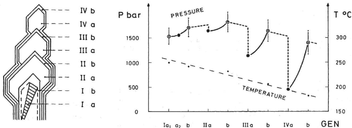
Figure 48 : The different textures of quartz crystal growth, in alpine fissure quartz from Val d'Illiez (Mullis, 1975) (left), with corresponding P-T conditions (right). A very similar pattern can be found in a study in the Appennines (Mullis, 1988d). Note that the scatter in homogenization temperature (vertical error bars in the right picture) is smaller than the fluid pressure drops. Black circles refer to CH 4 -rich inclusions, empty circles to H 2 O-rich ones.
