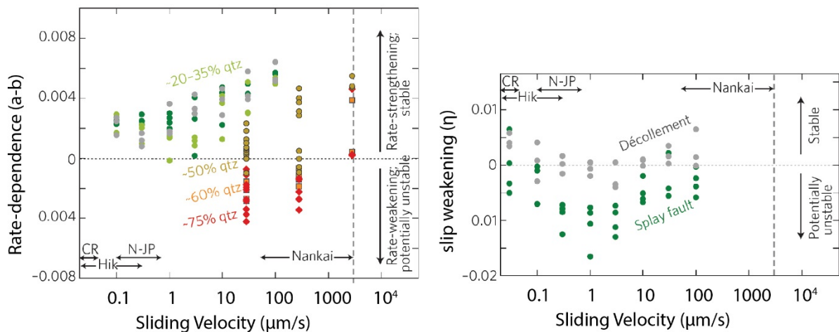
Figure 10 : Friction experiments results in Saffer and Wallace (2015), compiling results from Ikari et al. (2013) and Saito et al. (2013). (Left): In the traditional rate-and-state framework, the addition of quartz to clay mixture results in rate-weakening behavior. (Right): using a new formulation accounting for the decrease in friction coefficient with slip, the maximum of instability coincides with slip velocities of 1\text{-}10\mu\text{m/s} , i.e. the same magnitude as slow slip shown with double arrows. Grey and green points from (Ikari et al., 2013), orange and red ones from (Saito et al., 2013).
